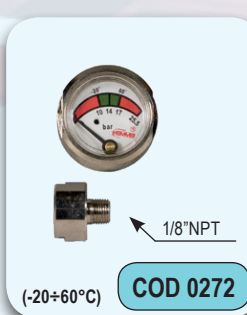
PRESSURE GAUGE Ø23 WITHOUT O-RING FOR FIRE SPRINKLER SYSTEMS
