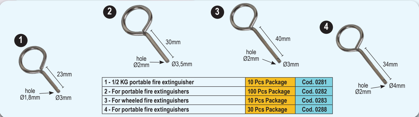
LOCKING PIN
